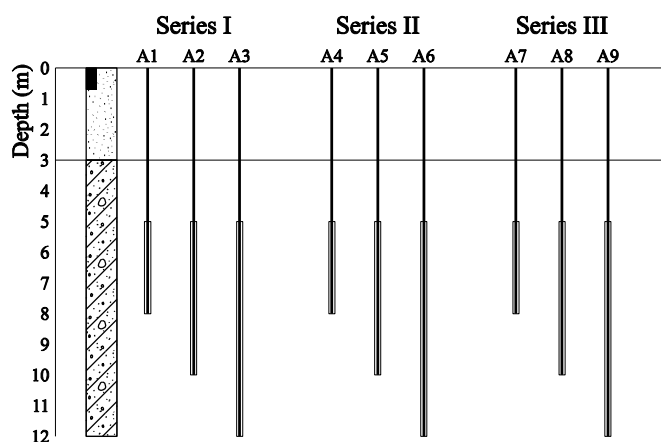
Figure 1. Anchor configuration. Principle
