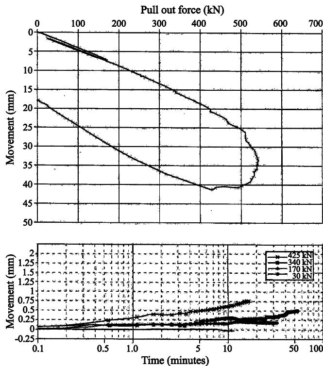
Figure 4. Pull out test.
