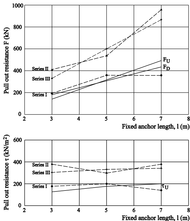
Figure 5. Pull out resistance of anchors as a function of the fixed length.
