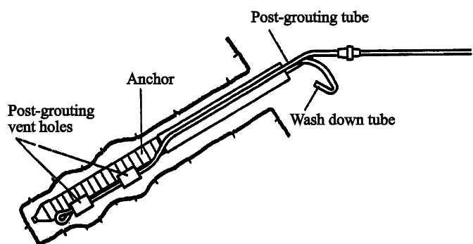
Figure 2. Post-grouting system (DYWIDAG).
